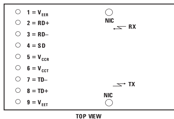
Figure 2. Pin-out.
