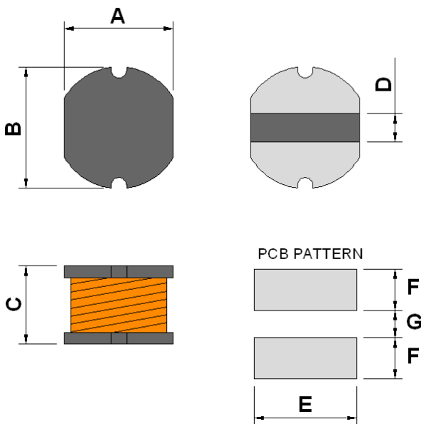
Dimensions [mm]
