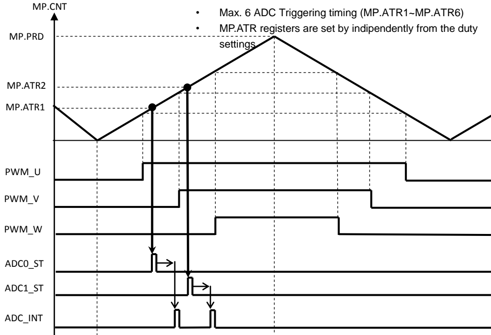
Figure 16.20. ADC Triggering Function Timing Diagram
