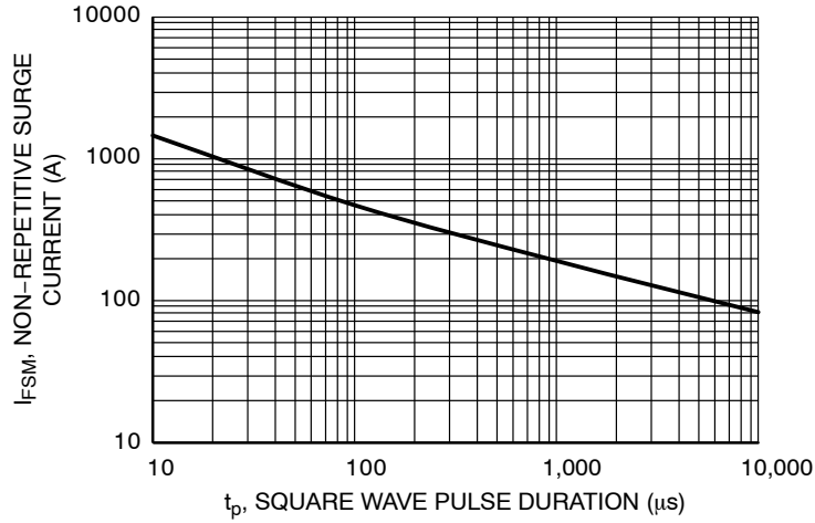
Figure 11. Typical Non-Repertitive Surge Current
